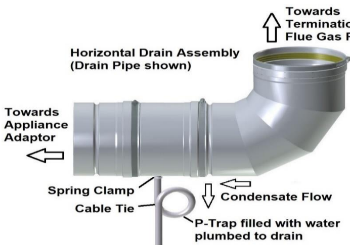
3/8" I.D. Silicone Tube Kit 2SVEDTKX Image 22
