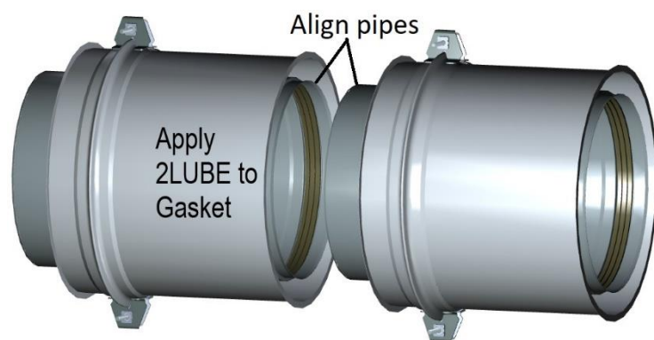
Double Wall ZV-Clamp Joint
