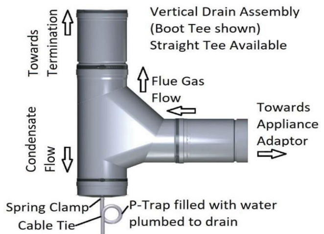
3/8" I.D. Silicone Tube Kit 2SVEDTKX Image 23
